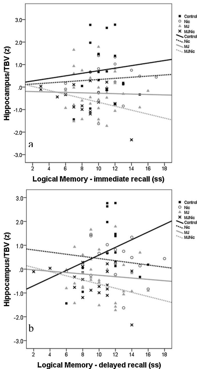
Fig. 2. Bivariate scatterplots with fit lines by group for hippocampal volumes (as TBV ratio z-score) with WMS-III logical memory (a) immediate recall scaled score (b) and delayed recall scaled score.
